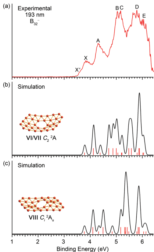
Fig. 2 Photoelectron spectrum of B_{32}^- at 193 nm (a) compared with the simulated spectra of the lowest-lying isomers of B_{32}^- ( C_2 , VI and VII) (b) and a low-lying isomer B_{32}^- ( C_j , VIII) (c) at the TD-PBE0/6-311+G(d) level. The simulated spectra were obtained by fitting the calculated VDEs (vertical red bars) with unit-area Gaussian functions of 0.05 eV half-width.
